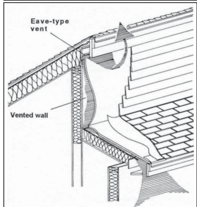
Figure 13. Providing adequate roof ventilation for a shed roof abutting a wall can be difficult. One option is to vent the roof air space into a vented wall.
