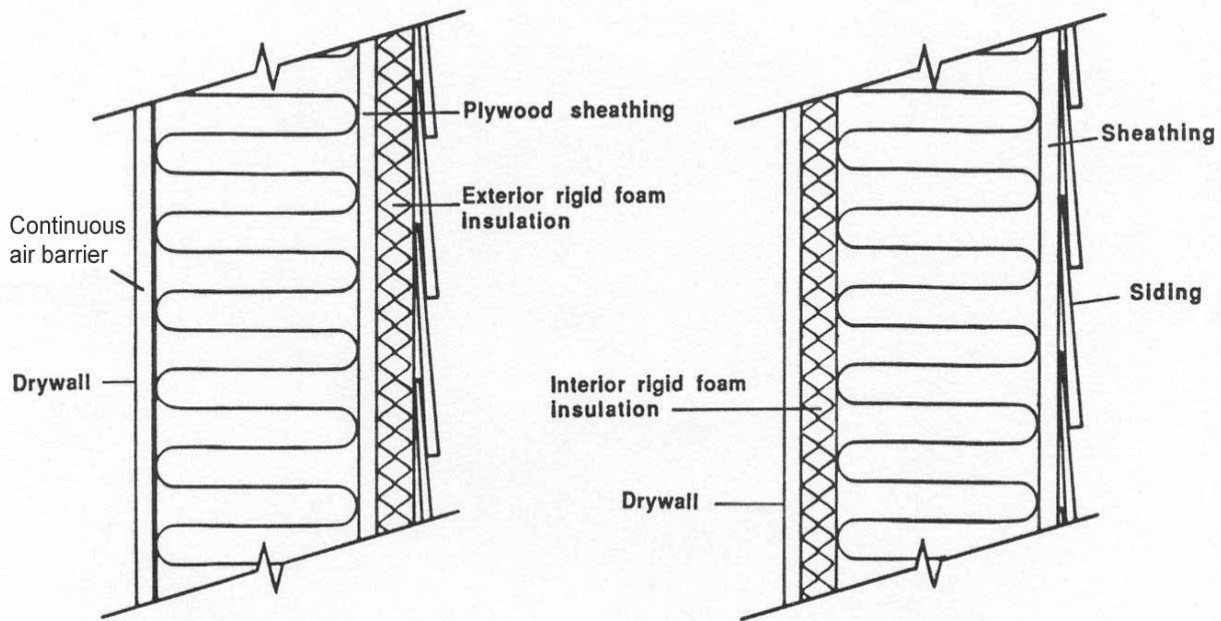
Figure 28. Rigid foam insulation can be installed on the inside or outside of the wall. While putting it on the outside is more common, more and more builders have begun putting it on the inside for various reasons. With a layer of rigid foam, the R-21 wall insulation requirements can be satisfied with a 2x4 wall.
