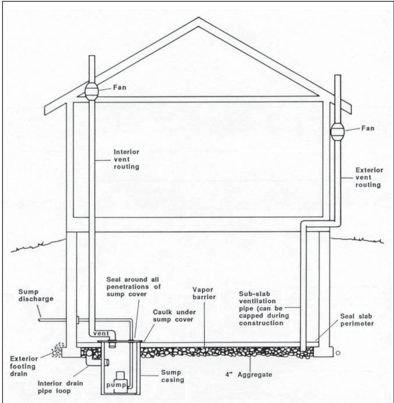
Figure 8. Designing a house to minimize the likelihood of radon problems—and to simplify future radon mitigation if it does become a problem—is quite easy.
