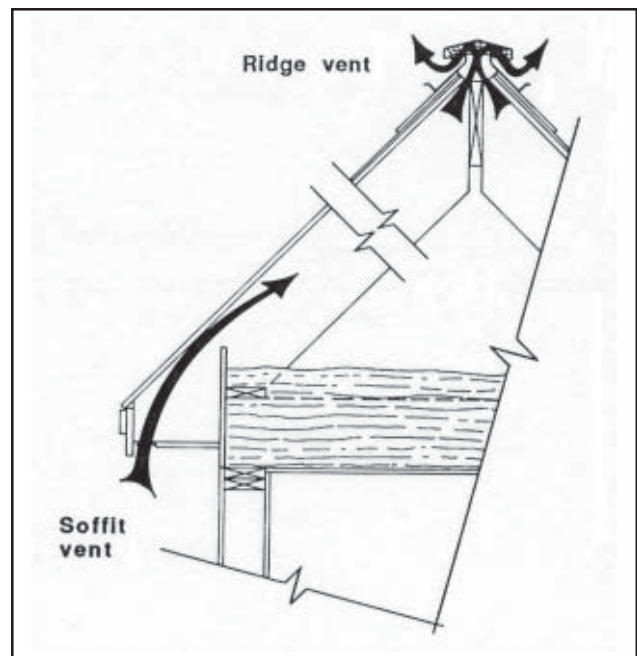
Figure 12. Optimal roof ventilation is provided with continuous soffit and ridge vents — whether for an unheated attic or cathedral ceiling application.
