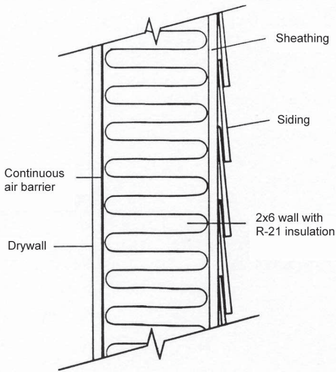
Figure 27. Standard R-21 wall section using 2x6 studs and cavity-fill fiberglass or cellulose insulation.
